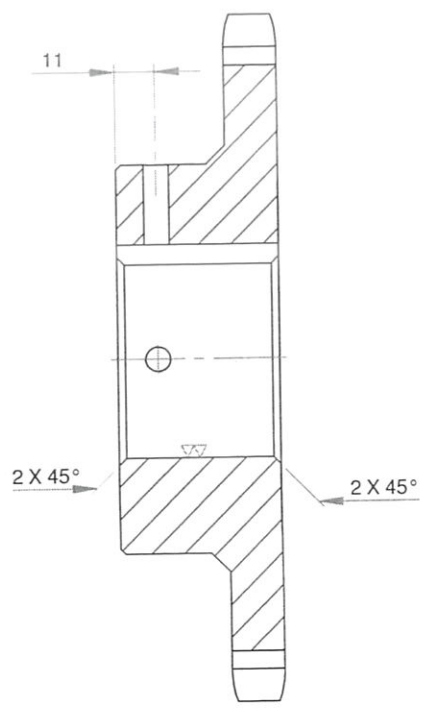
SECTION C-C SCALE 1 : 2
