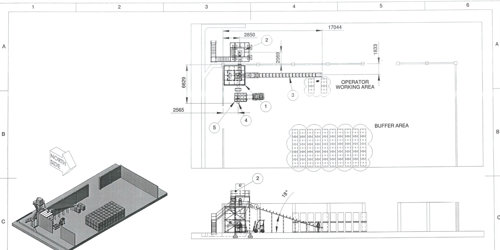
ISOMETRIC VIEW
