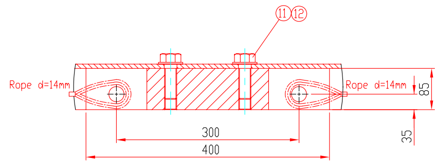
DETAIL B SCALE 1 : 2
