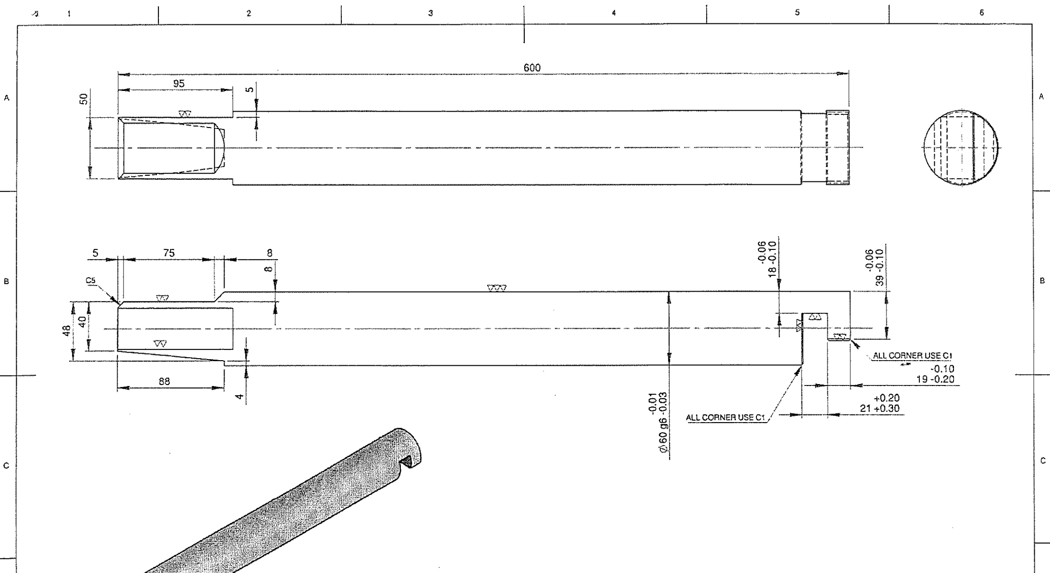
ISOMETRIC VIEW #NB: WIGHT= 11,201 KG
