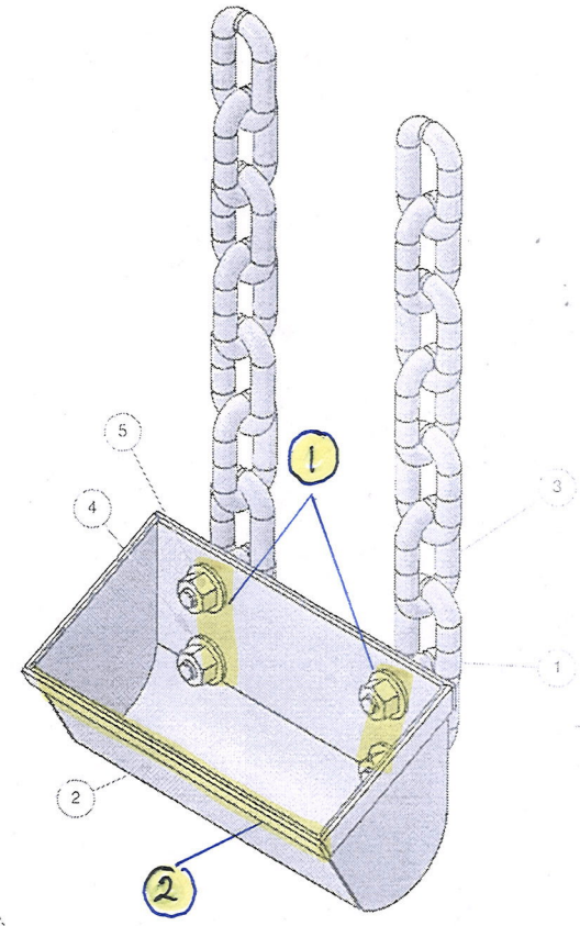
ISOMETRIC VIEW SCALE 1:8
