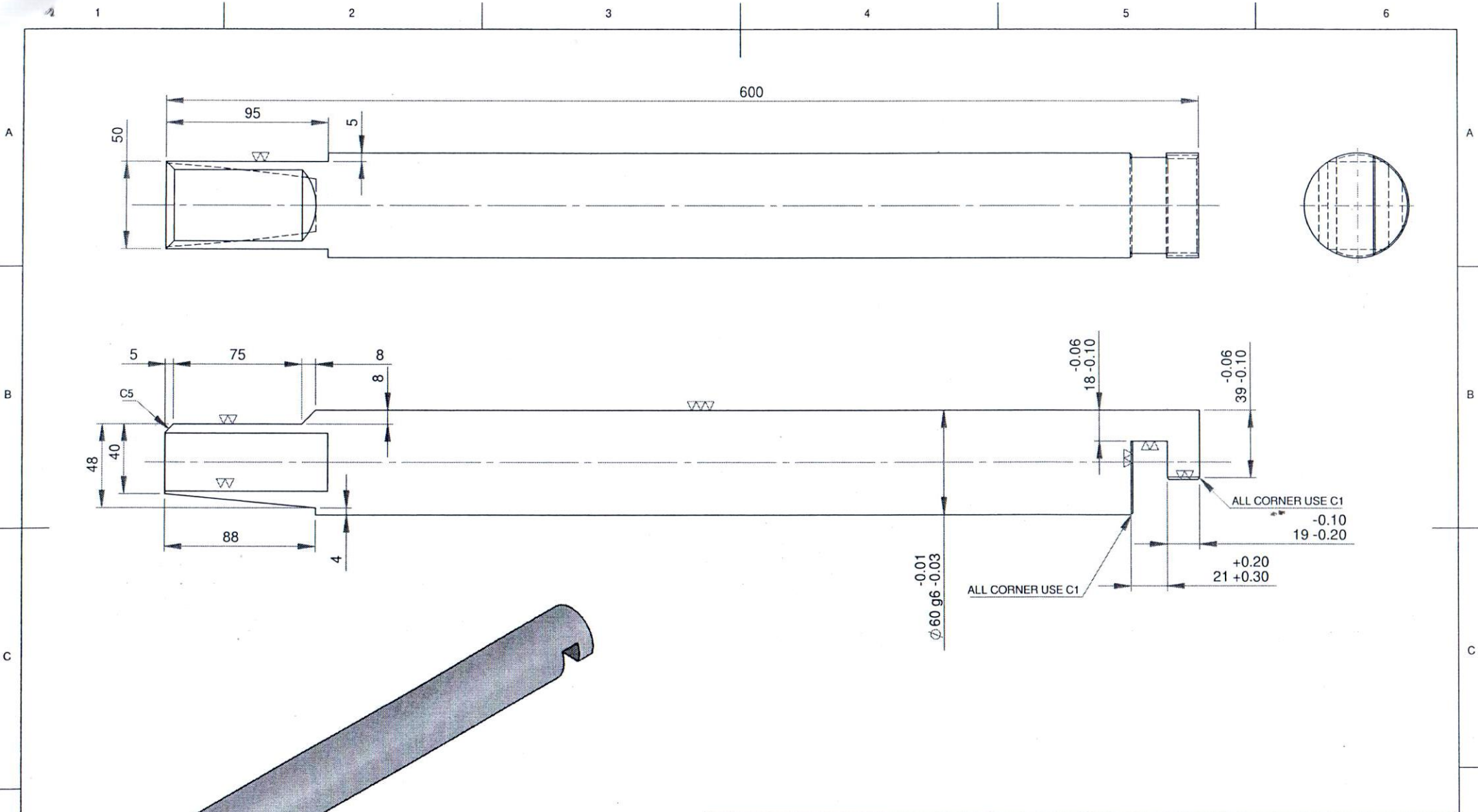
ISOMETRIC VIEW #NB: WIGHT= 11,201 KG
