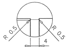
DETAIL D
